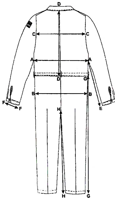
Fig 3 - Coverall Measurements
