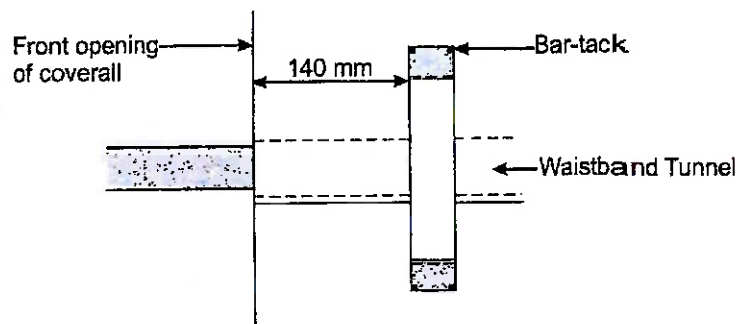
Fig 6 - Belt Loops
