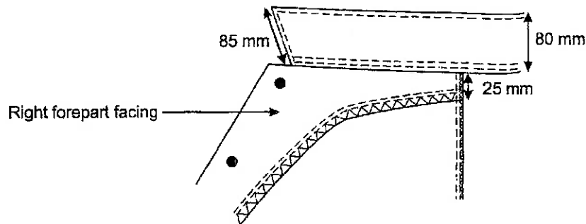
Fig 4 - Collar
