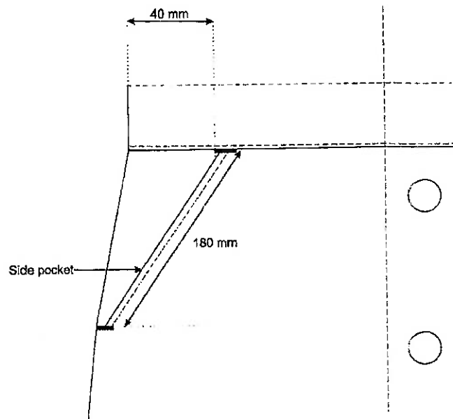
Fig 12 - Side Pockets
