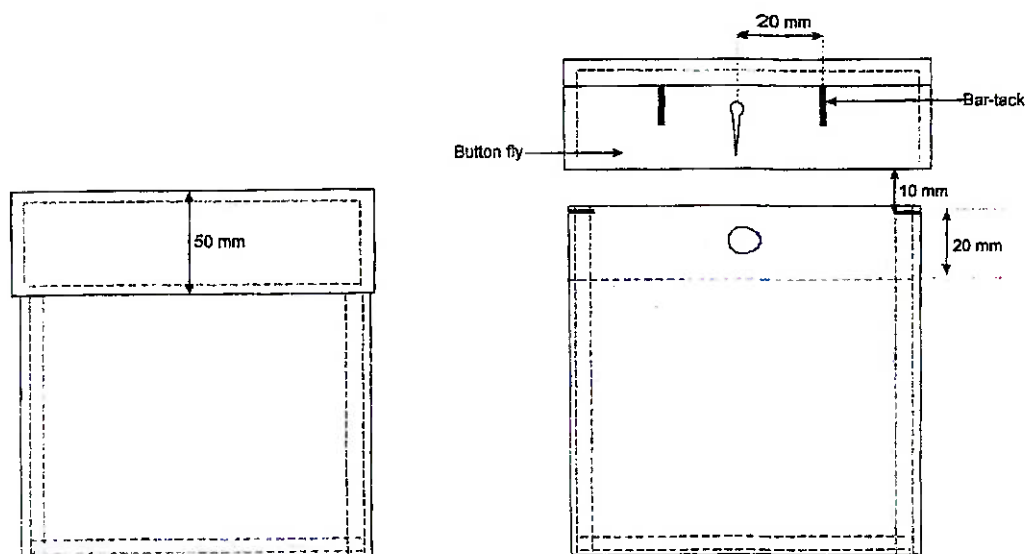
Fig 11 - Breast Pockets
