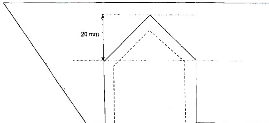
Fig 10 - Shoulder Straps
