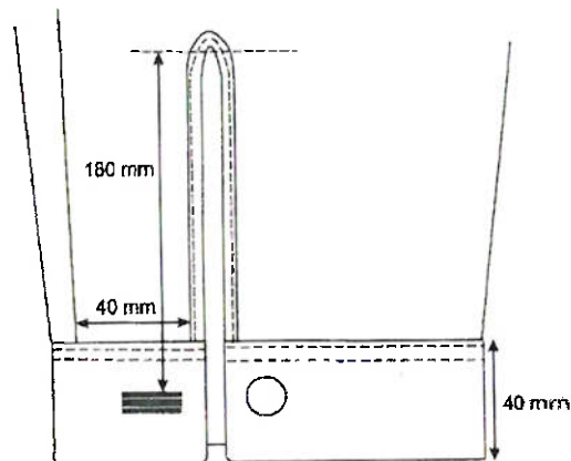
Fig 7 - Cuffs
